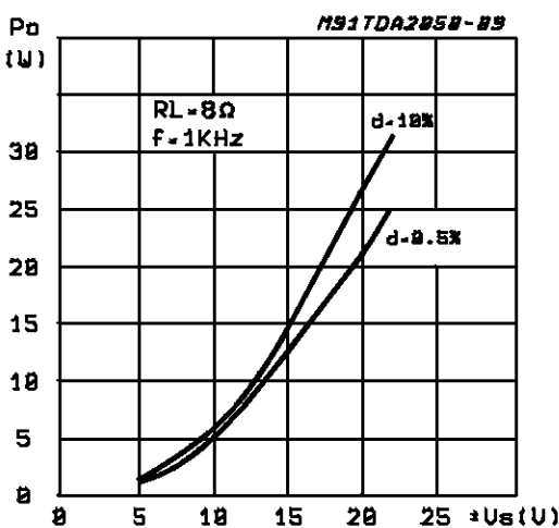
Figure 5: Output Power vs. Supply Voltage
